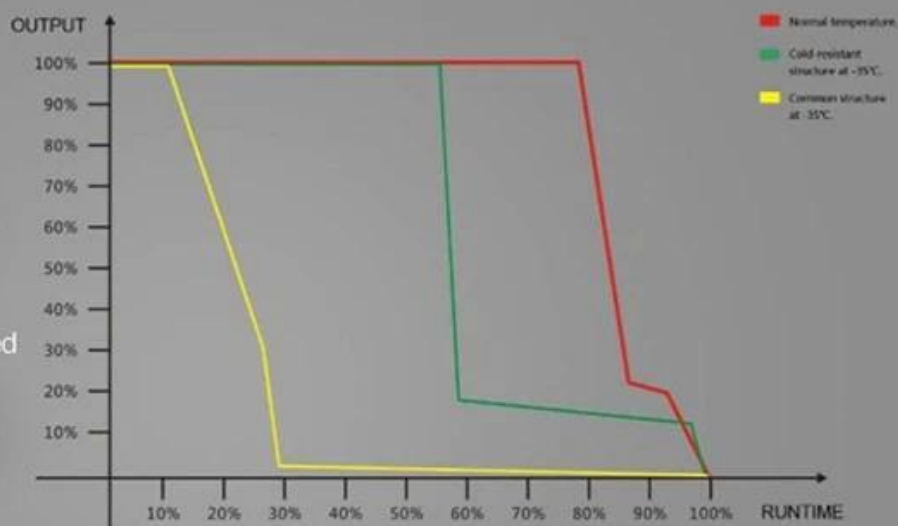
Runtime curves of 18650 Li-ion rechargeable battery
